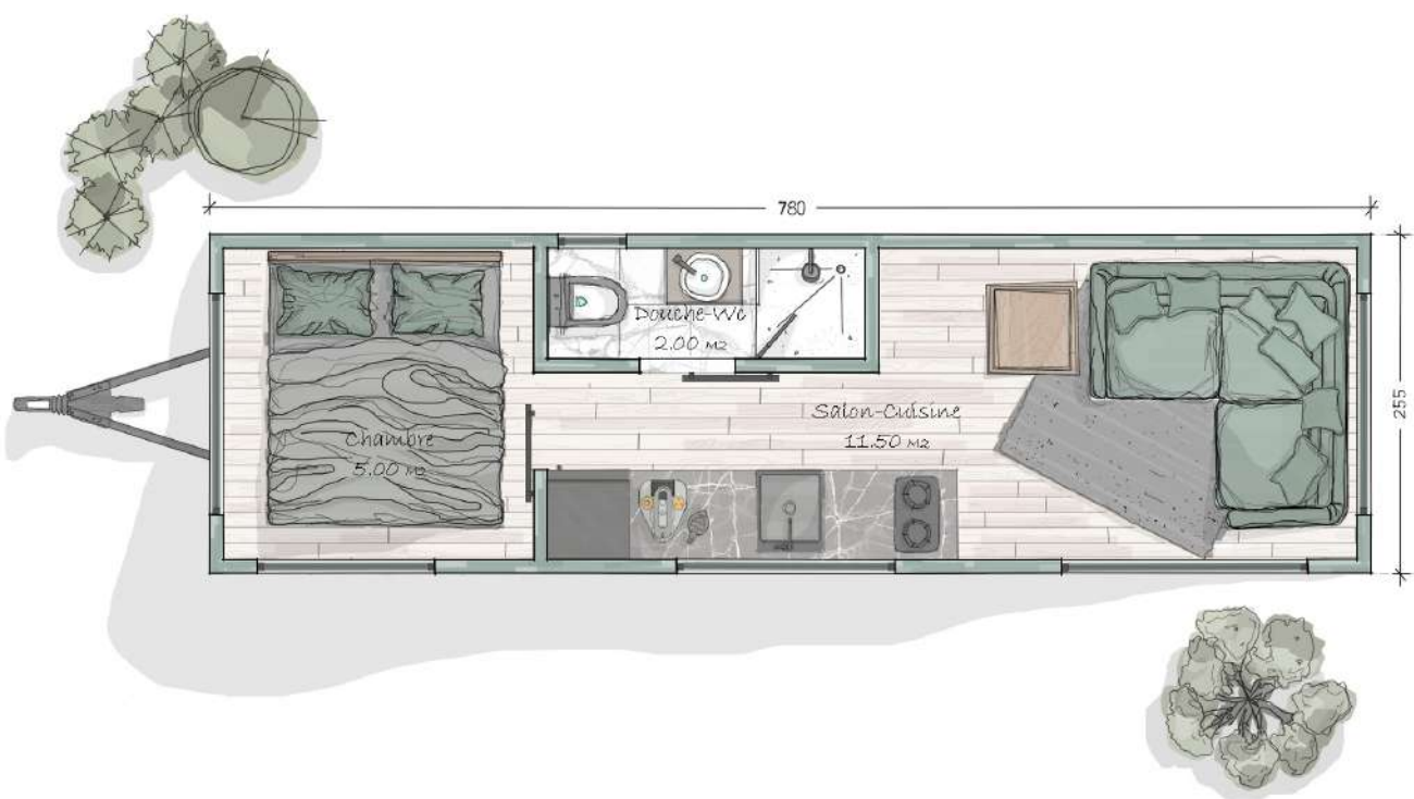
PLAN SUN-LIKYA (20m 2 )
